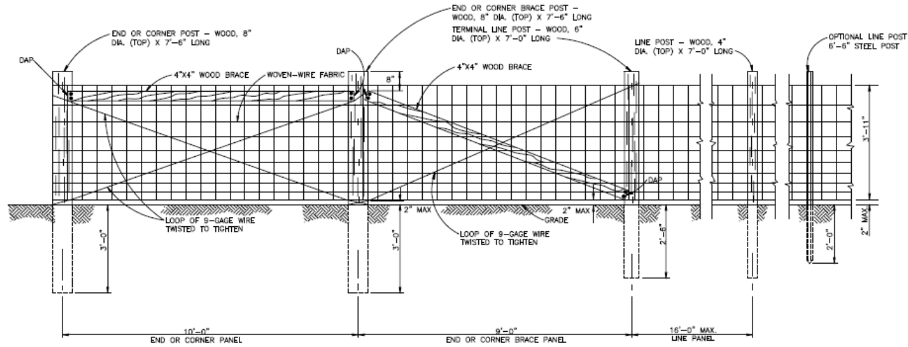
TYPICAL LAYOUT-WOVEN-WIRE FENCE NO SCALE
