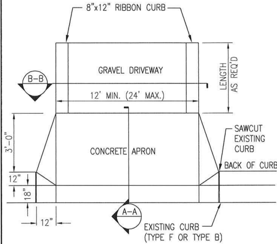
DRIVEWAY APRON NOT TO SCALE
