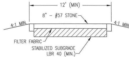
SECTION B-B NOT TO SCALE
