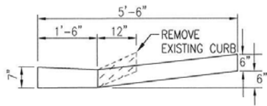
SECTION A-A NOT TO SCALE
