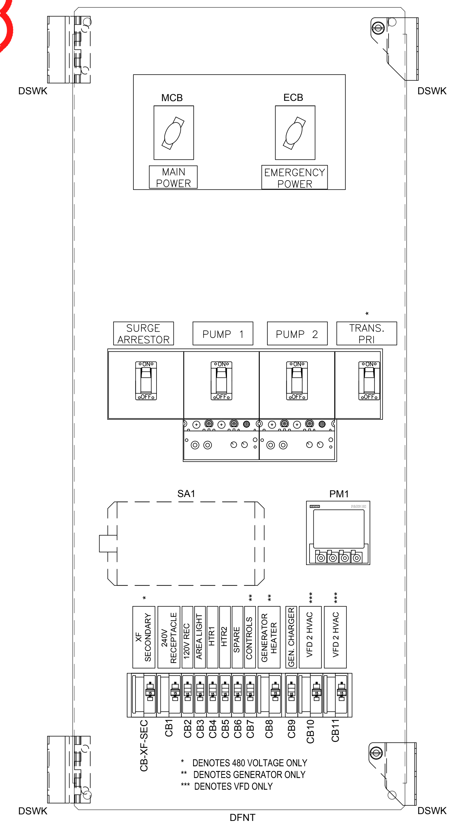
Dead Front Layout
