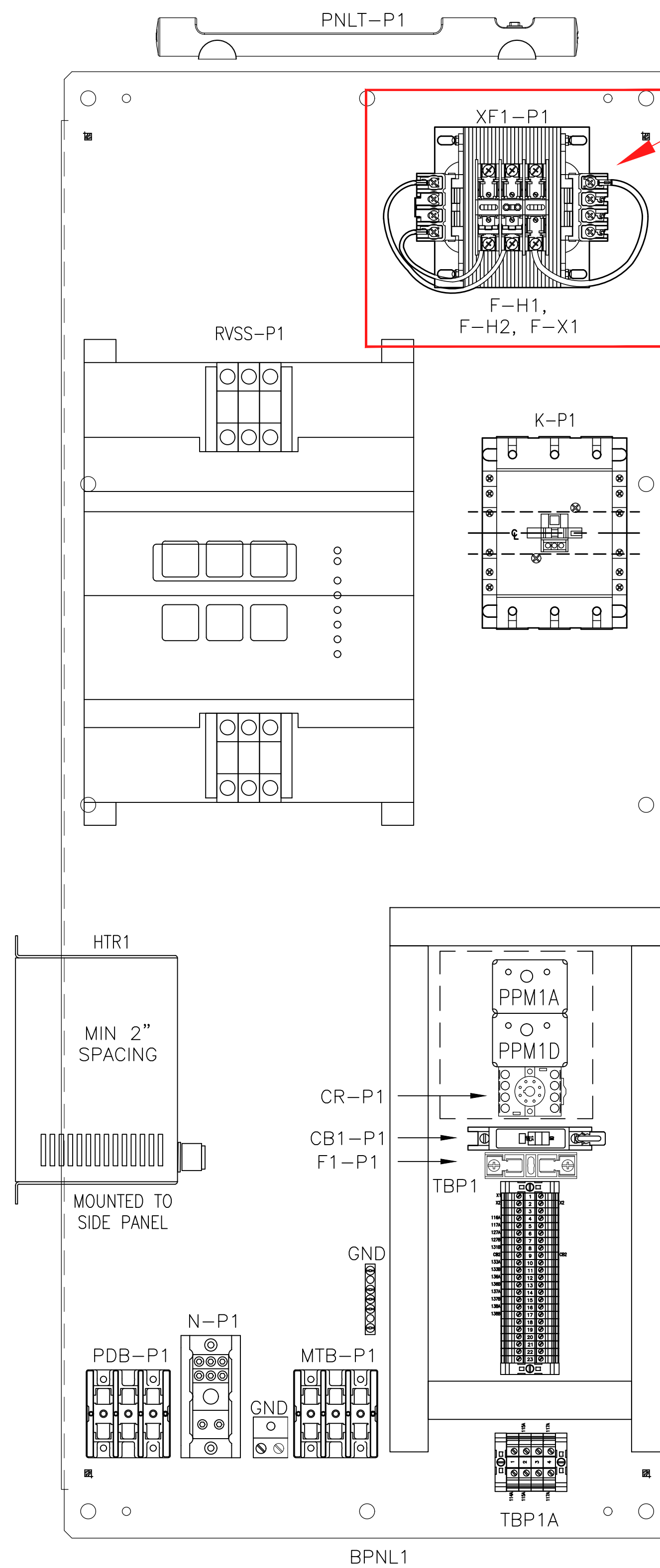
PUMP ENCLOSURE LAYOUT
