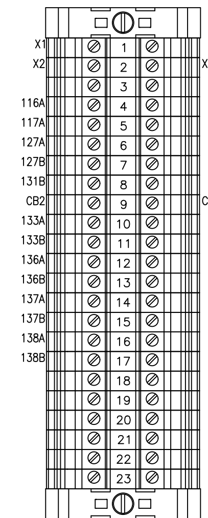
TBP1 LAYOUT
