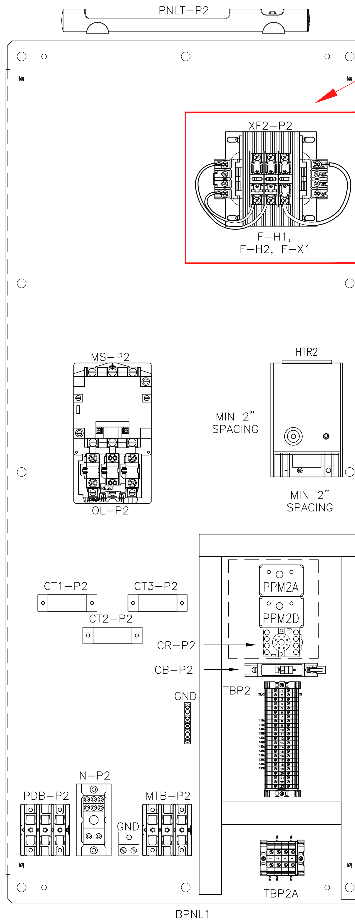
PUMP ENCLOSURE LAYOUT
