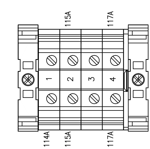
TBP2A LAYOUT UT10 3044160 - 4 D-UT2.5/10 3047028 - 1
