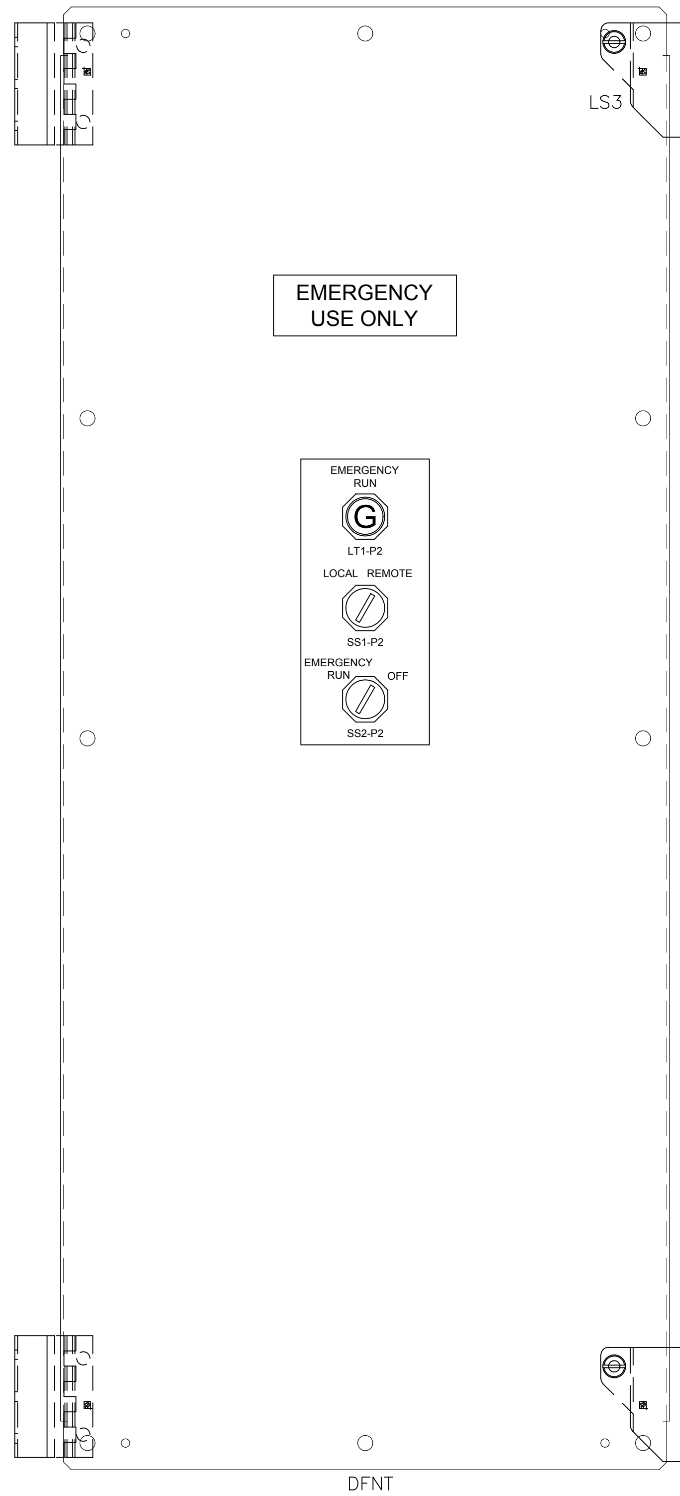
DEADFRONT LAYOUT
